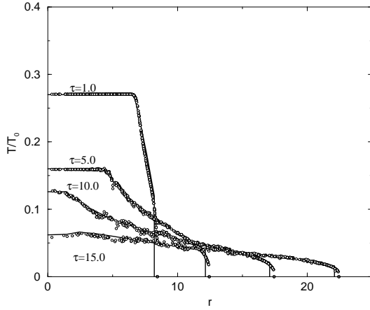
Figure 10. Temperature profile of a cylindrically symmetric flow with longitudinally scaling expansion, shown as a function of r = \sqrt{x^2 + y^2} . The SPH results at \eta = 0 (circles) are compared with the numerical solution obtained by a space-fixed grid method [41]. The SPH calculation has been performed in full 3D.
