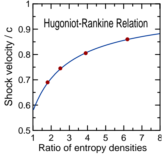
Figure 13. Test of Hugoniot-Rankine relation. The circles are results of SPH calculations with different initial conditions, and the full curve is Eq. (109).
