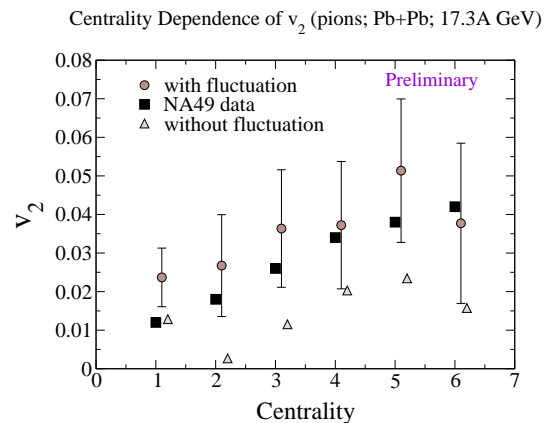
Figure 24. Centrality dependence of v_2 for pions for Pb+Pb collisions at SPS. The data are from NA49 [62].
