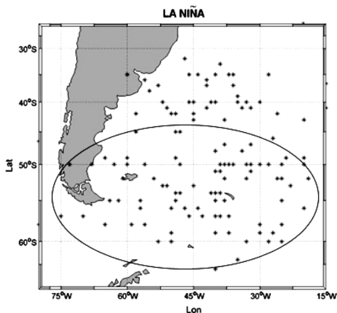
FIGURE 9 – Region of 67 cyclogenesis during La Niña (may 2007 to march 2008). The ellipse indicates a higher occurrence of extratropical cyclones below latitude 47.5 S (region I).
