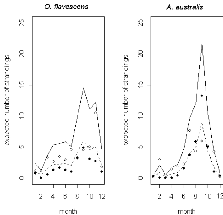
Figure 3. Expected number of strandings \hat{\mu} by month for the southern region 1 (—●) and northern region 2 (---○), for sea lions (left) and fur seals (right) in south Brazil. The average number of observed strandings for the southern (○) and northern (●) regions are also included.
